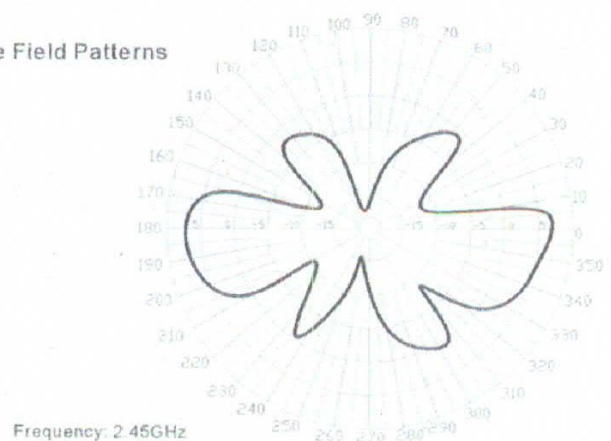
H-Plane Field Patterns
