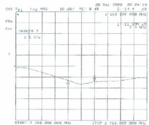
Return Loss
