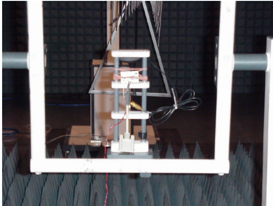
Picture 3 : Setup for radiated emission tests
