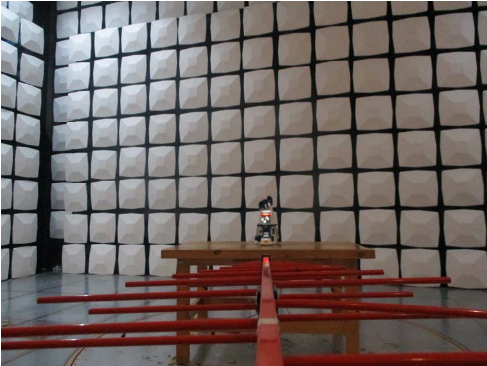
Radiated Emission Below 1GHz Panthera D View
