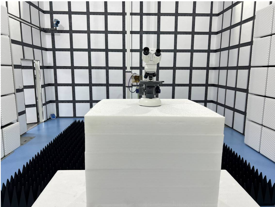
Radiated Emission - Front View (1GHz-3GHz)
