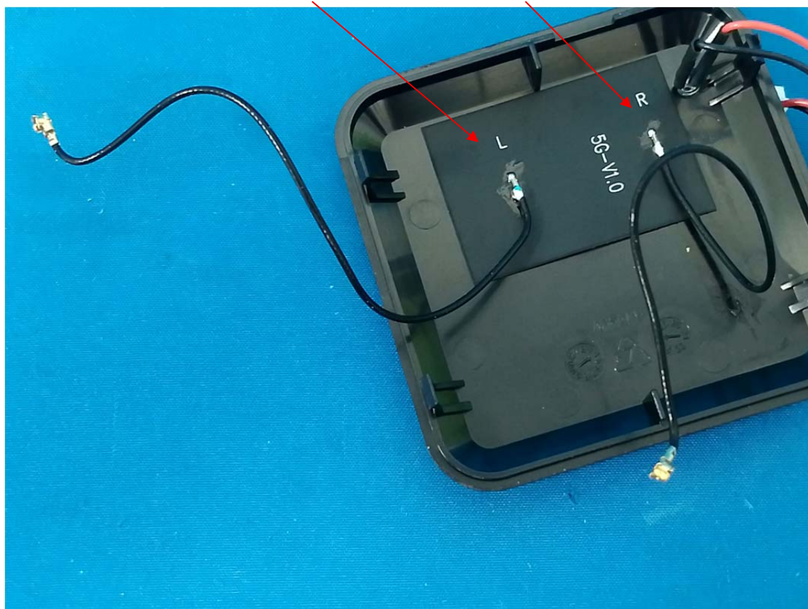
Chain 0 Antenna
