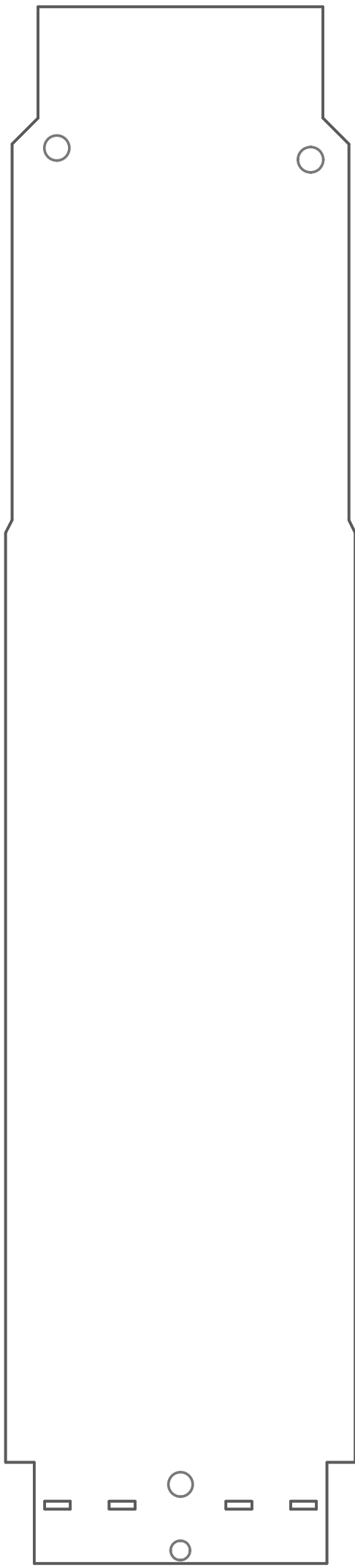
VHF-30HHM Wireless Transmitter Bottom Overlay
