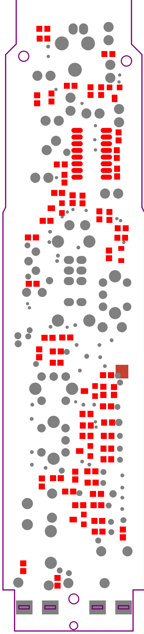
VHF-30HMH Wireless Transmitter Bottom Solder and Paste Mask
