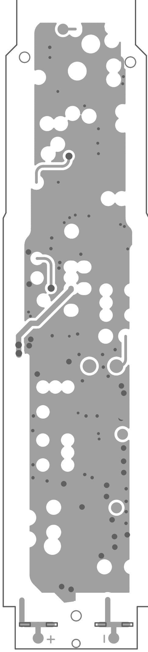
VHF-30HHM Wireless Transmitter Bottom layer
