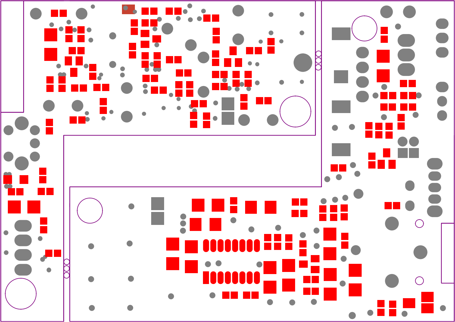
VHF-30BP Wireless Transmitter Top Solder and Paste Mask
