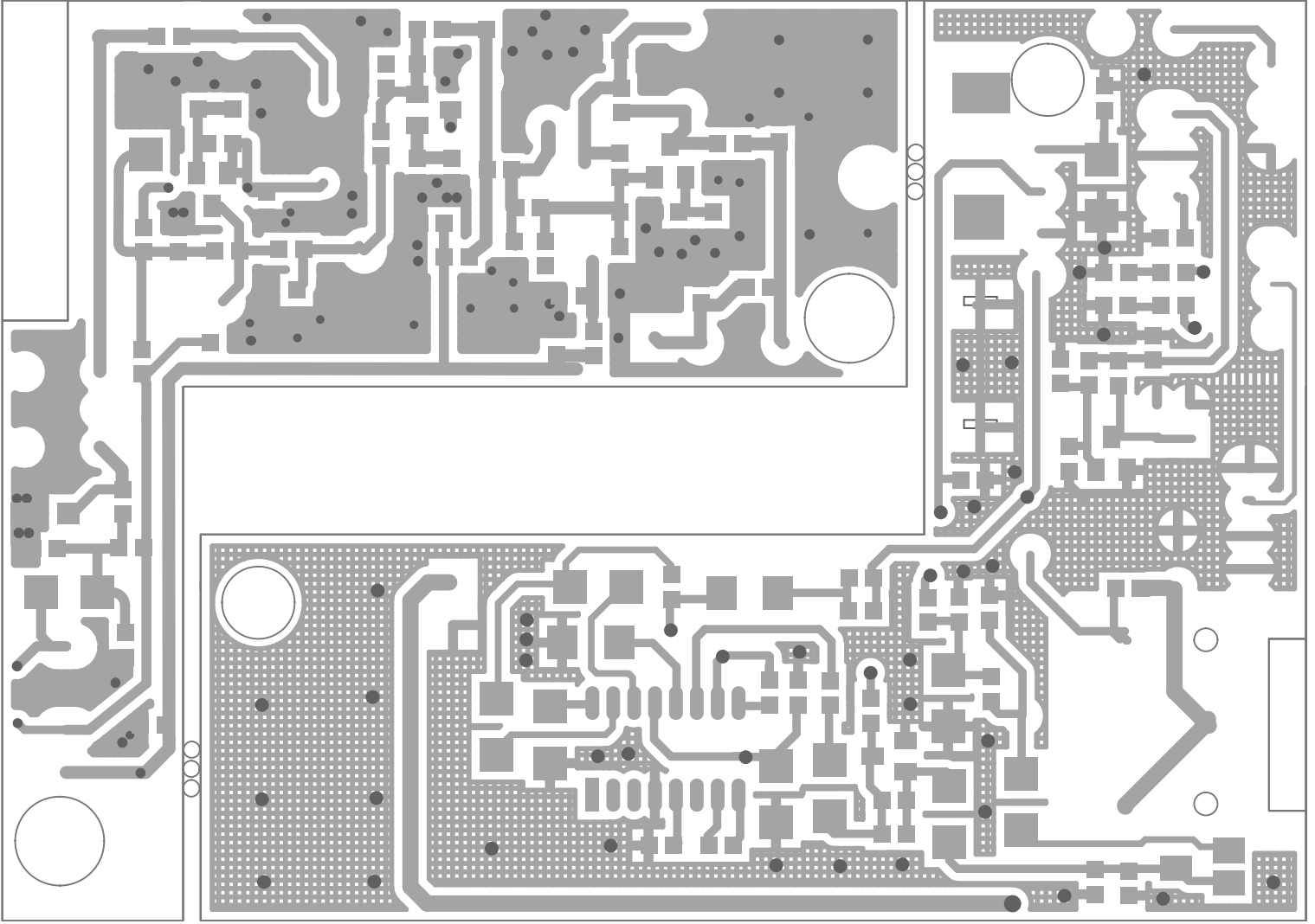
VHF-30BP Wireless Transmitter Top Layer
