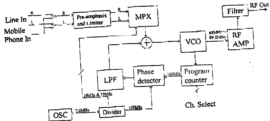
MP-1688 Block Diagram
