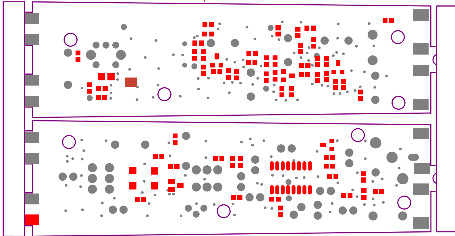
HT-V20 Transmitter Top Solder and Paste Mask
