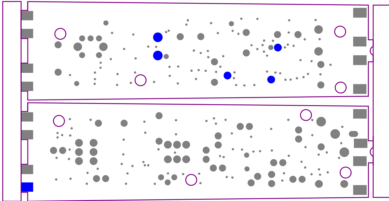
HT-V20 Transmitter Bottom and Paste Mask
