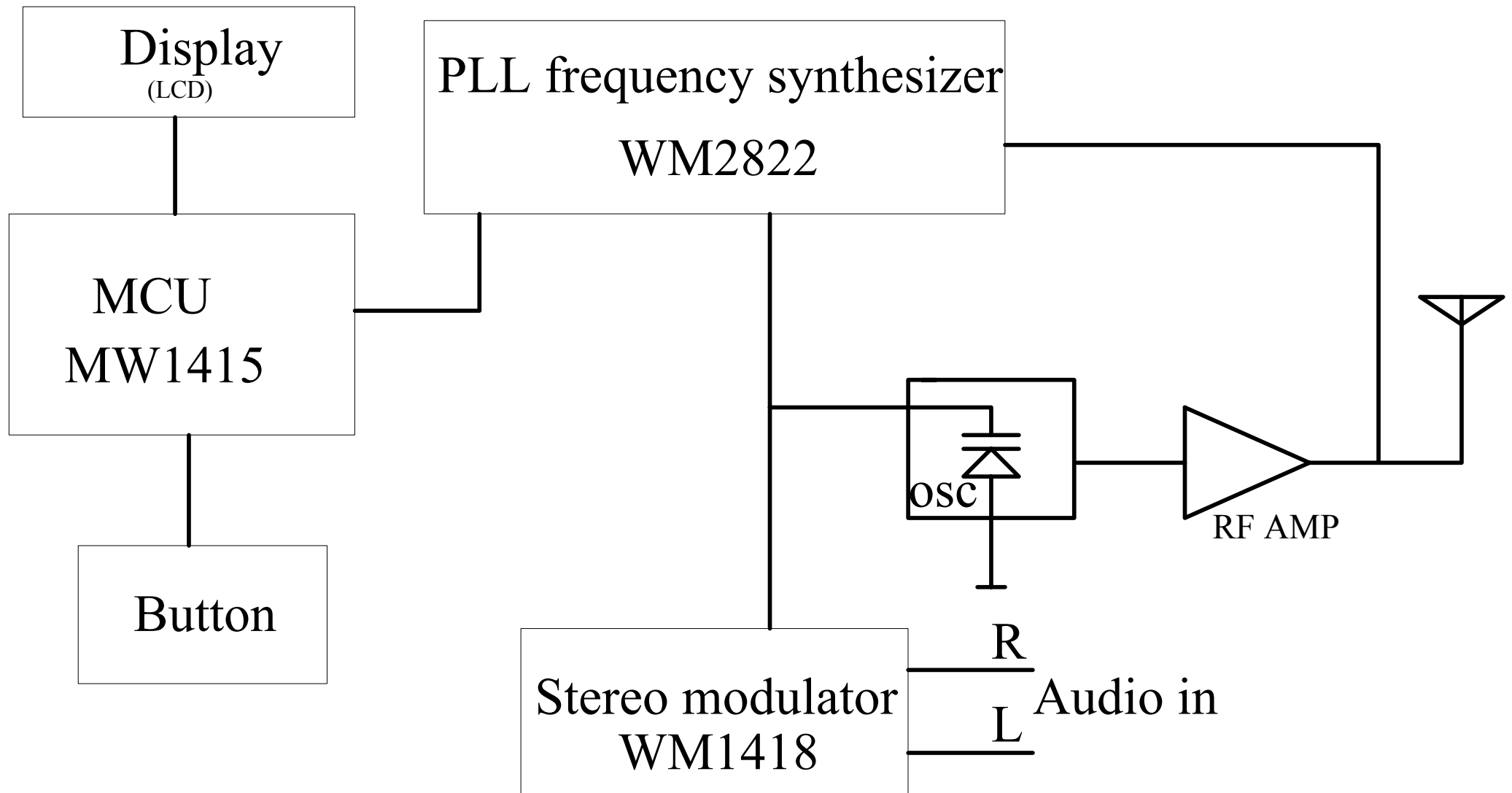
CF2028F BLOCK DIAGRAM
