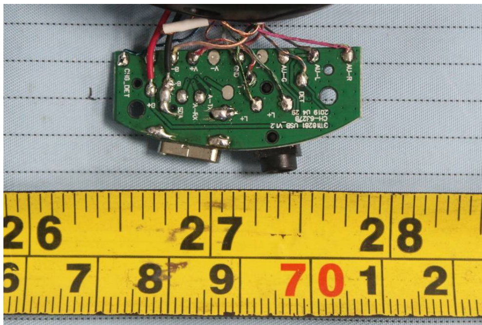
EUT –USB & AUX Board Bottom View
