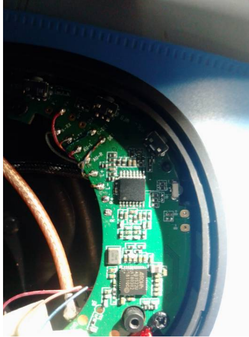
EUT – Main Chip View
