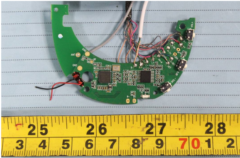
EUT – Main Board Top View
