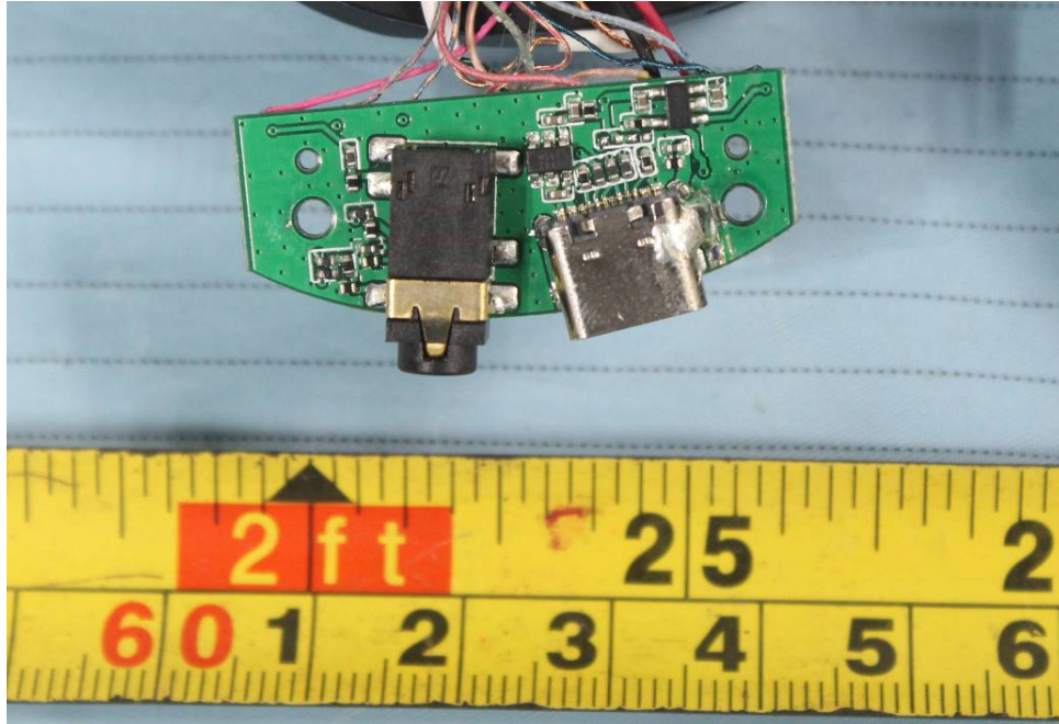
EUT – USB & AUX Board Top View
