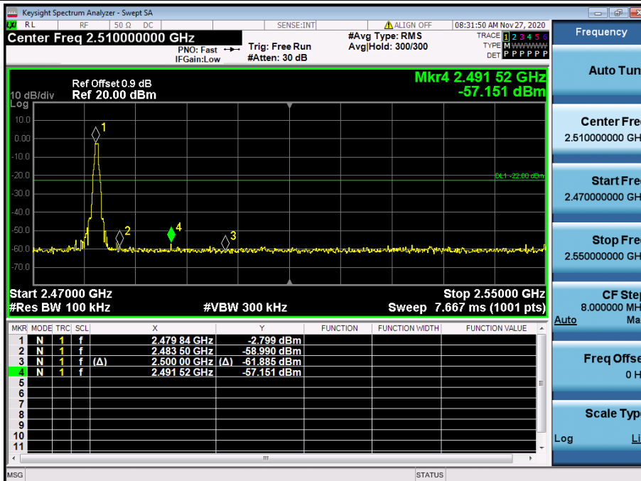
DH5_Ant1_High_2480
