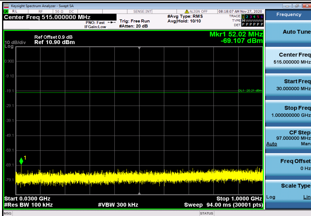
DH5_Ant1_2402_30~1000
