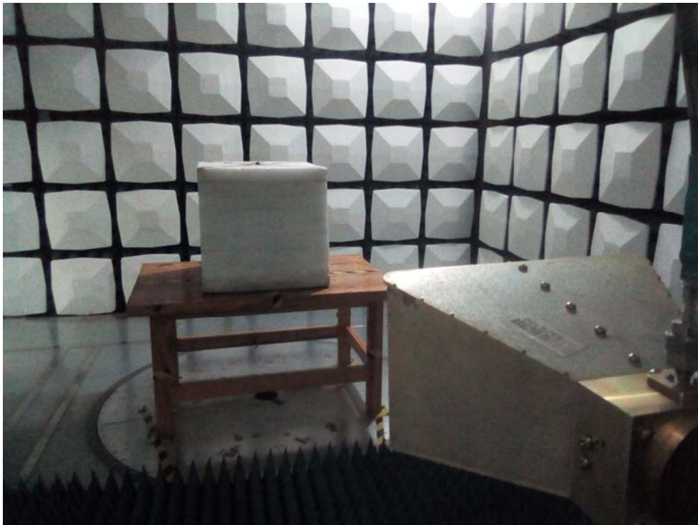
Radiated Emission Above 1GHz 1M View
