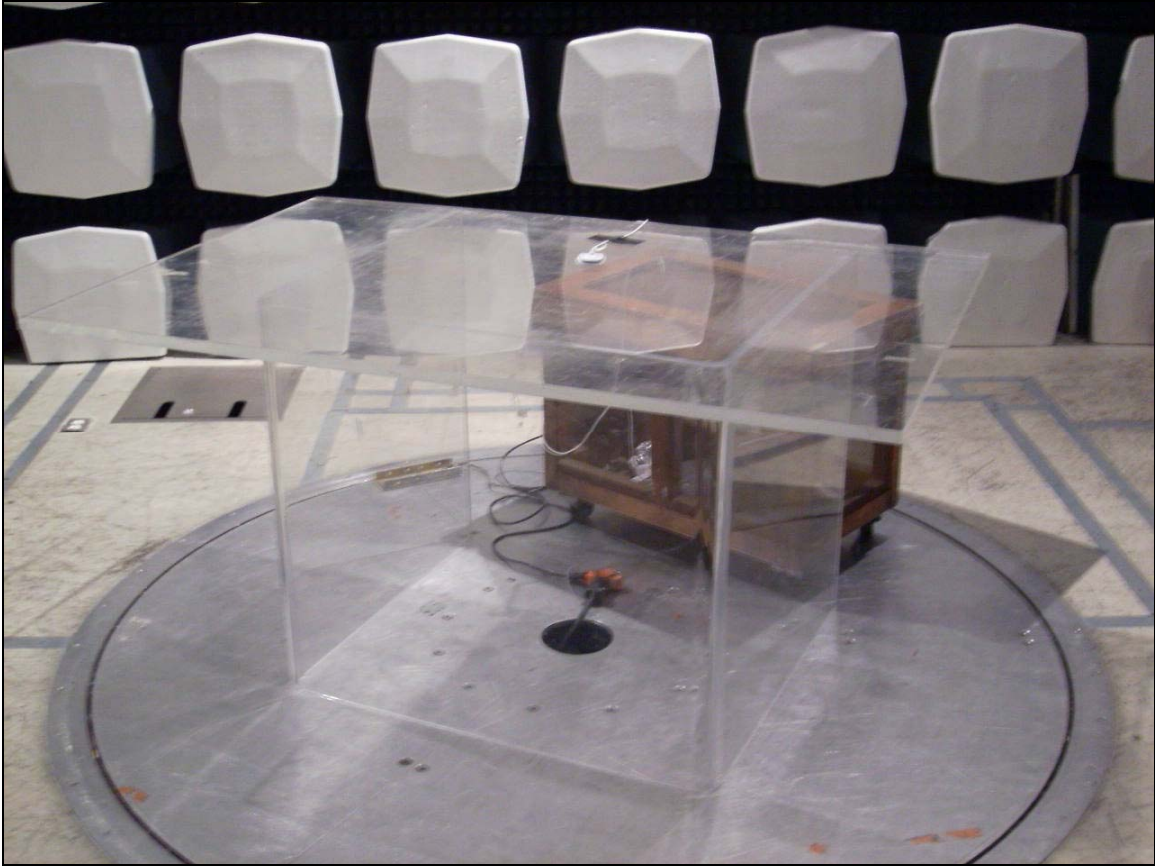
Photograph 2. Test Setup
