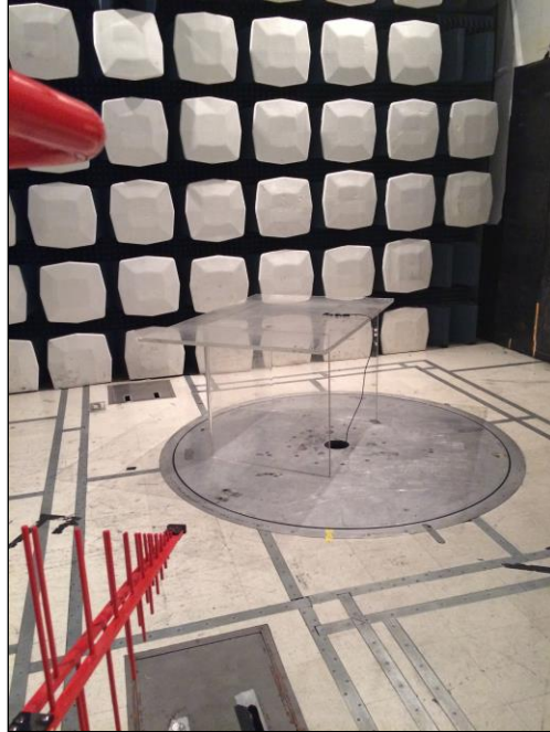
Photograph 4. Radiated Spurious Emissions, Test Setup, 1
