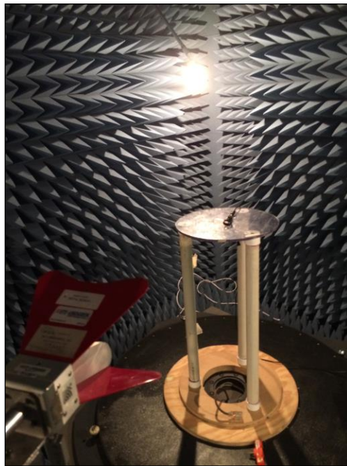
Photograph 5. Radiated Spurious Emissions, Test Setup, 2
