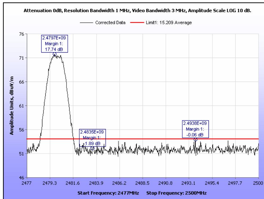
Plot 25. Radiated Restricted Band Edge, High Channel, Peak under Average
