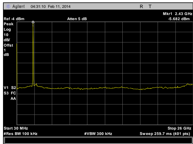
Plot 26. Conducted Spurious Emissions, Low Channel, 30 MHz – 26 GHz
