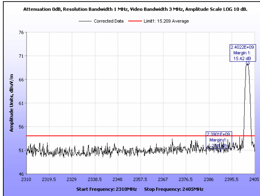
Plot 24. Radiated Restricted Band Edge, Low Channel, Peak under Average
