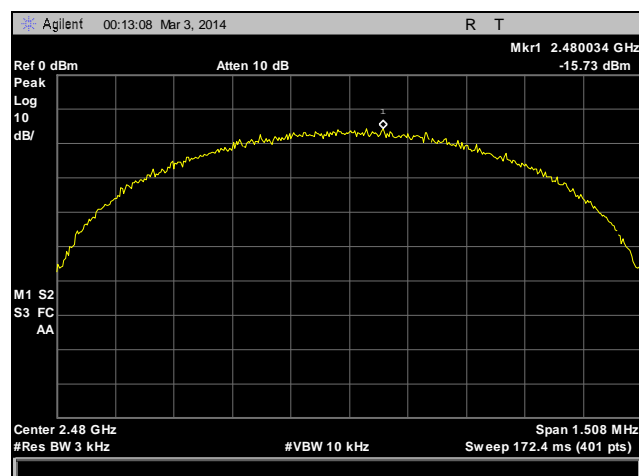
Plot 33. Peak Power Spectral Density, High Channel
