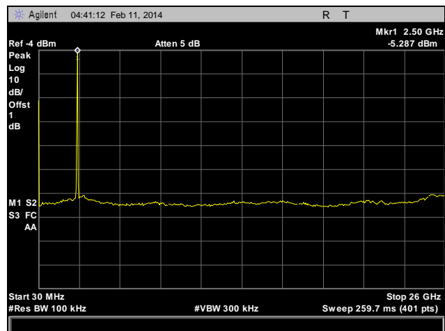
Plot 28. Conducted Spurious Emissions, High Channel, 30 MHz – 26 GHz
