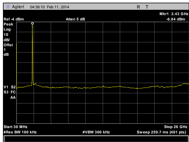
Plot 27. Conducted Spurious Emissions, Mid Channel, 30 MHz – 26 GHz
