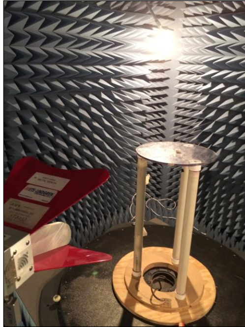
Photograph 2. Radiated Spurious Emissions, Test Setup, 1
