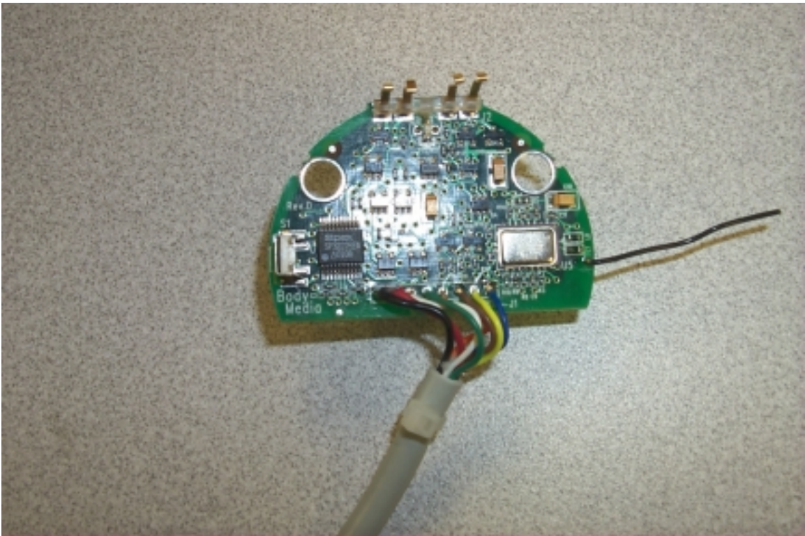
Side A of internal PC board
