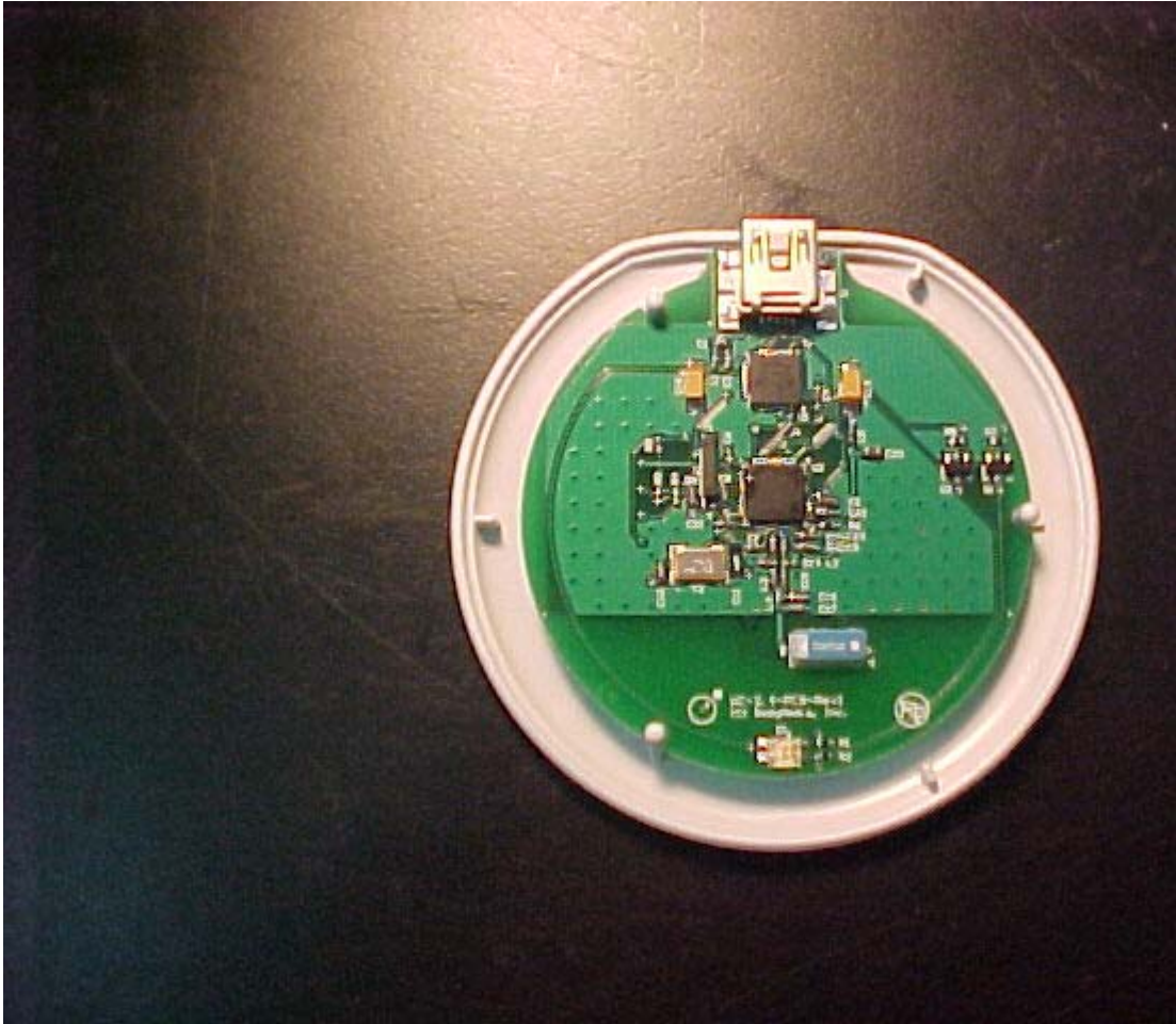
PCB top view
