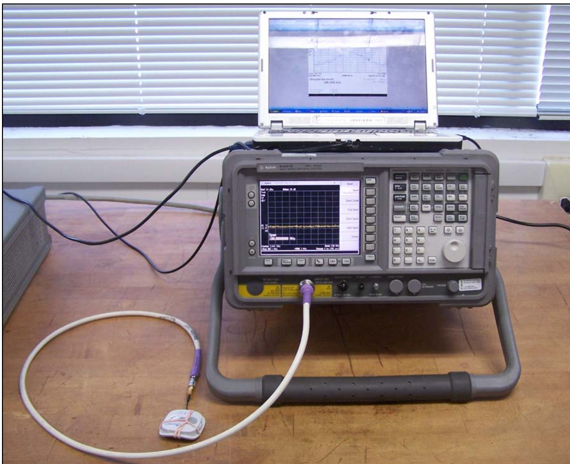
Conducted Power Test Setup
