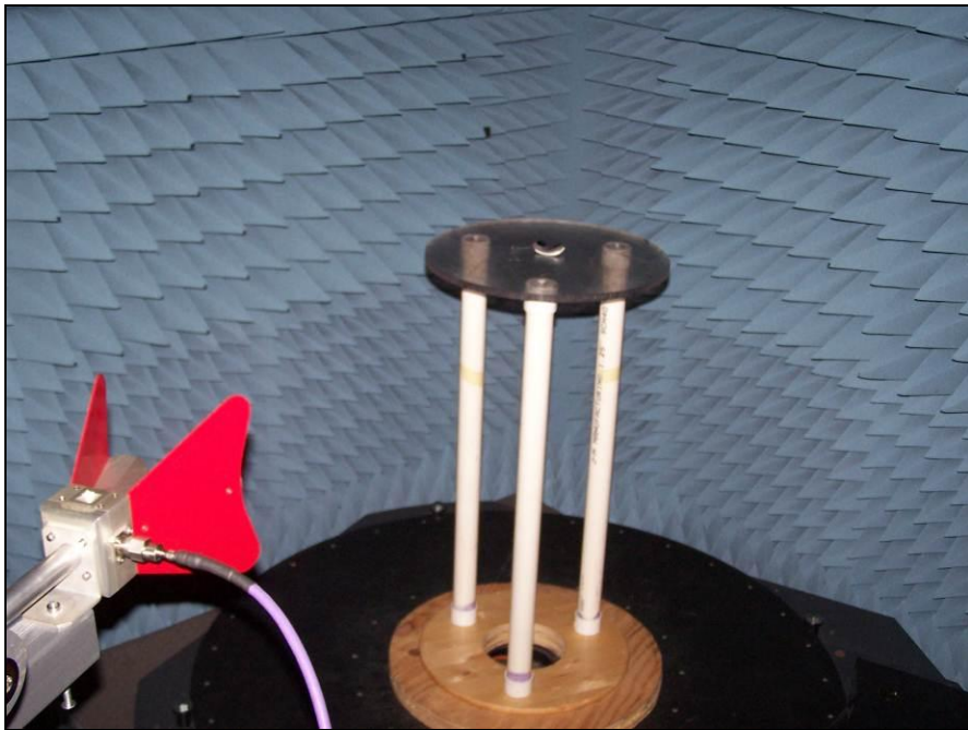
Photograph 4. Radiated Spurious Emissions, Test Setup 2
