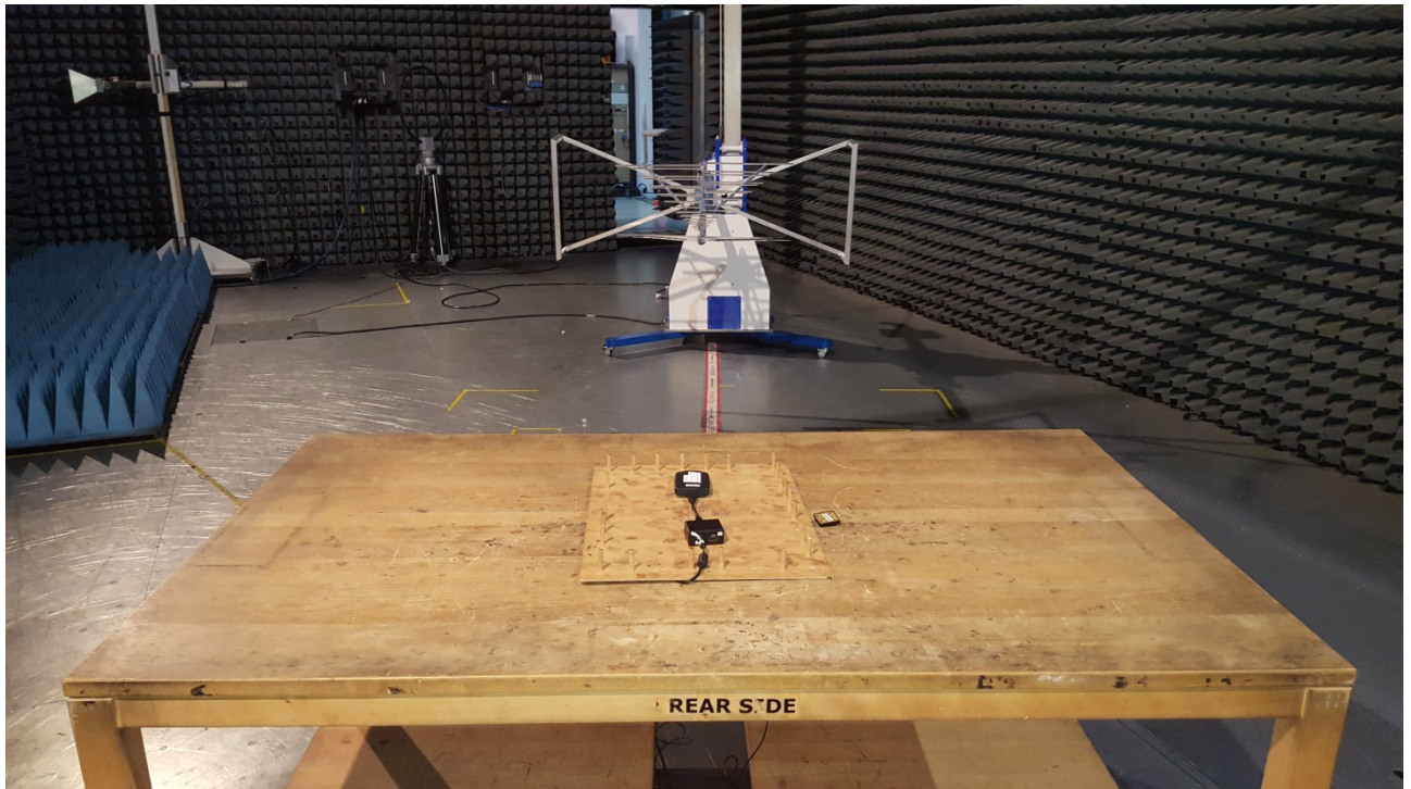
Photo 3: Test setup for radiated measurements in semi-anechoic chamber, 30 MHz to 1 GHz
