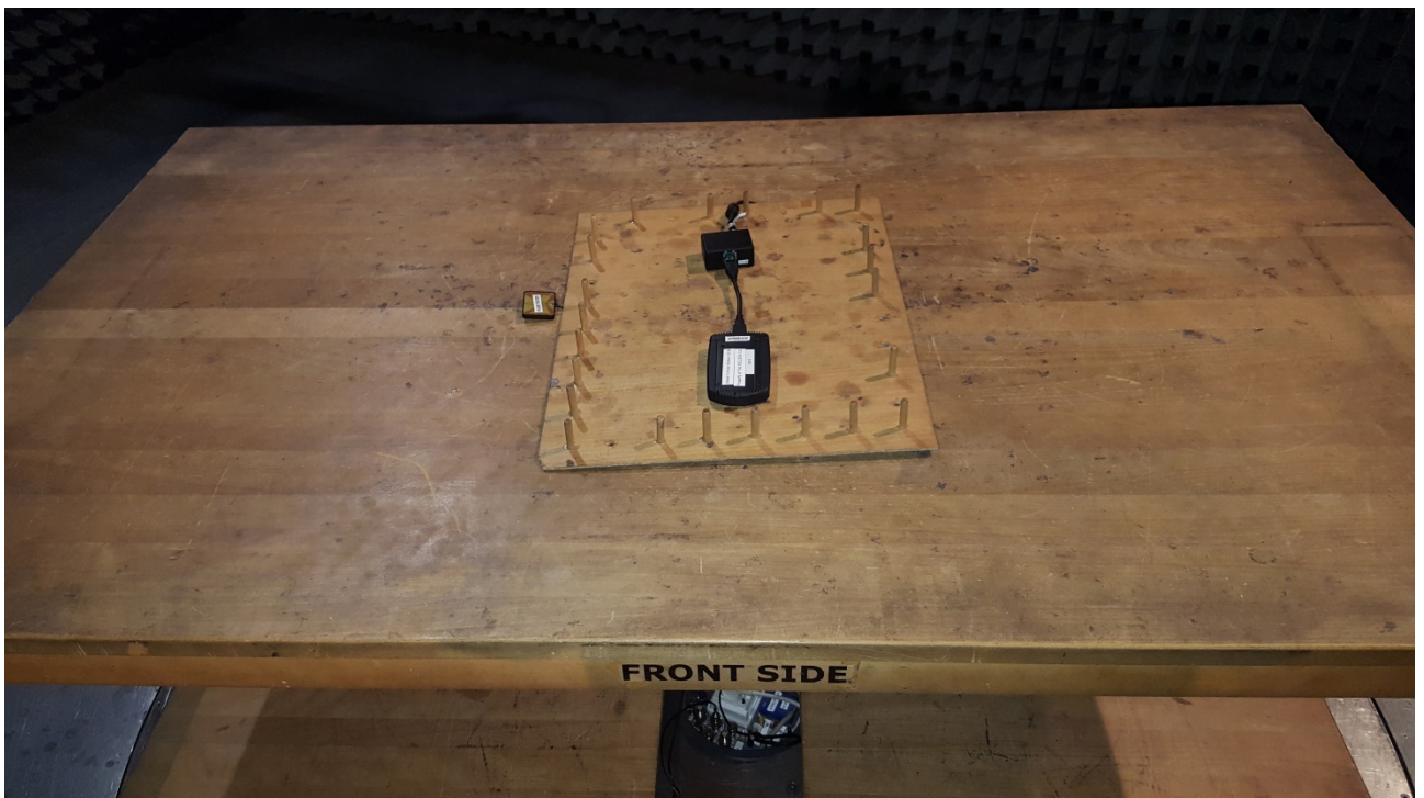
Photo 2: Test setup for radiated measurements below 1 GHz, detailed view
