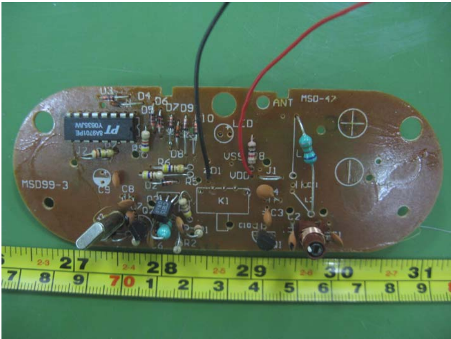
EUT – Main Board Top Component View
