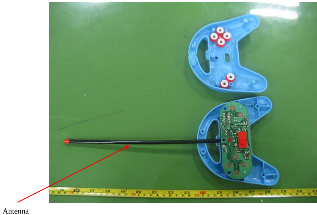
EUT – Main Board Top Component View
