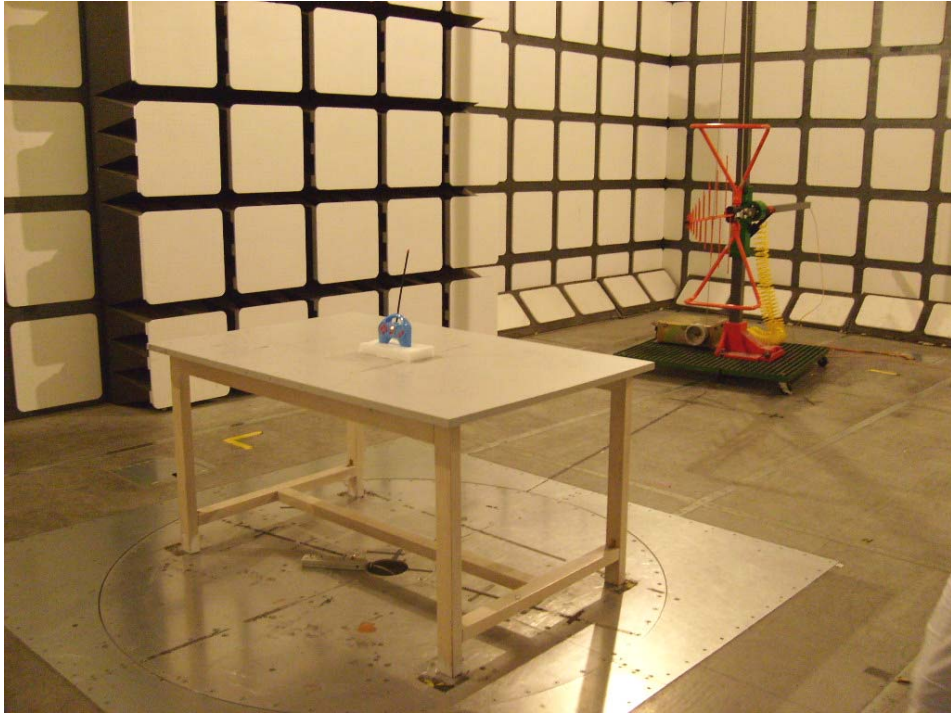
Radiated Emissions with EUT antenna vertical orientation –Rear View
