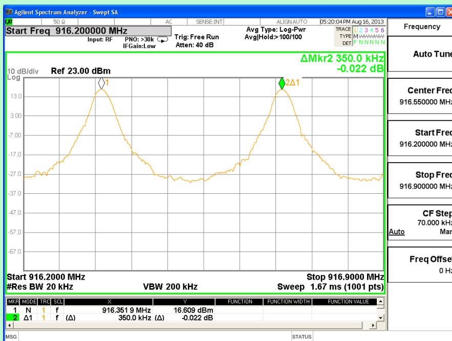
Channel 27 and 28
