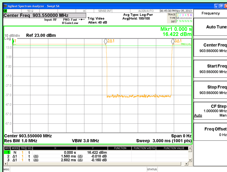
Channel 1 (903.55 MHz)
