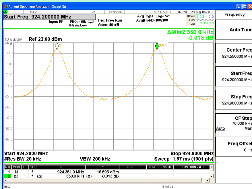
Channel 46 and 47
