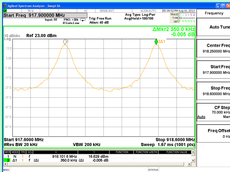
Channel 32 and 33
