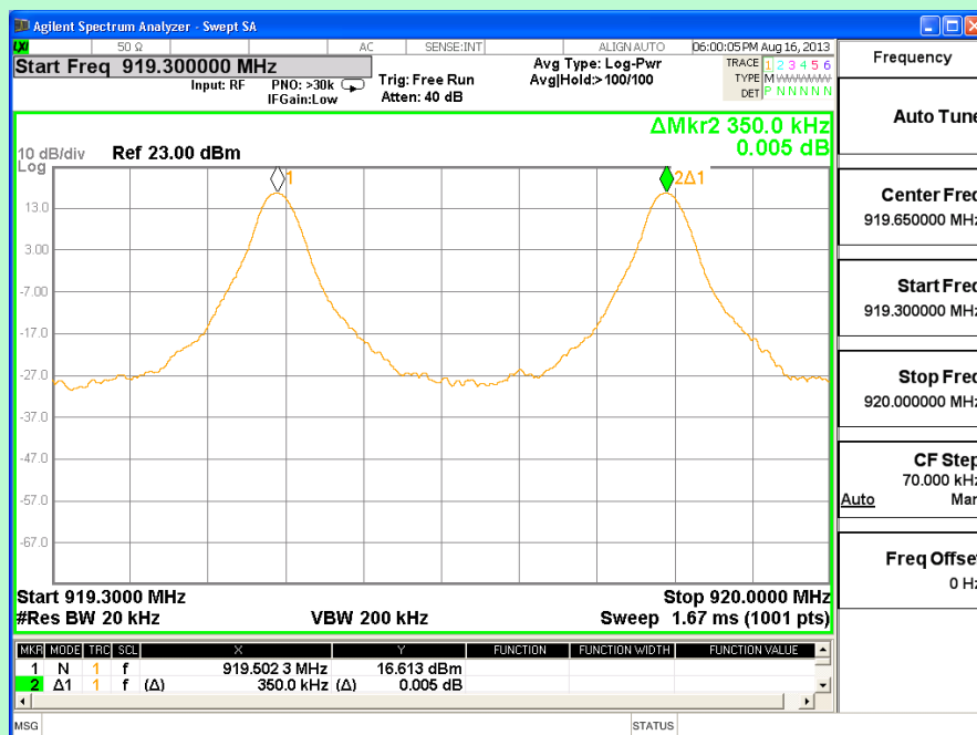
Channel 36 and 37
