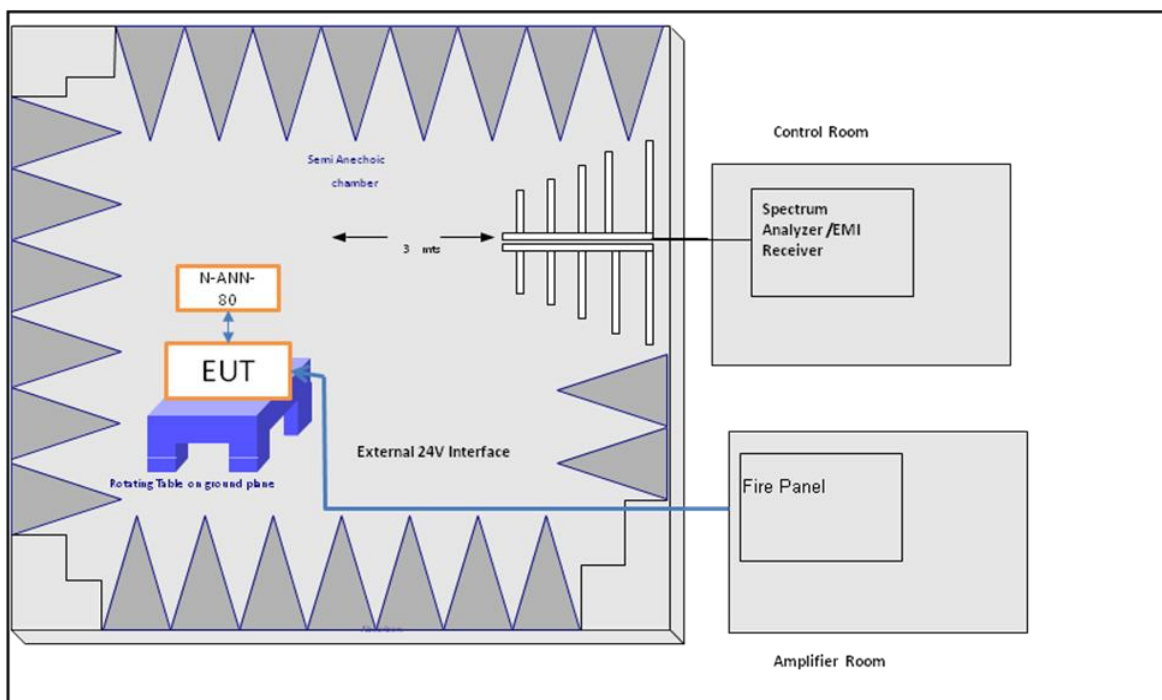
Radiated Emission Test Setup
