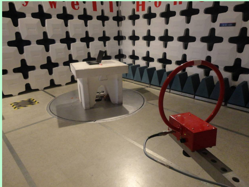
Radiated Emission Setup – 9KHz to 30MHz [ Parallel]
