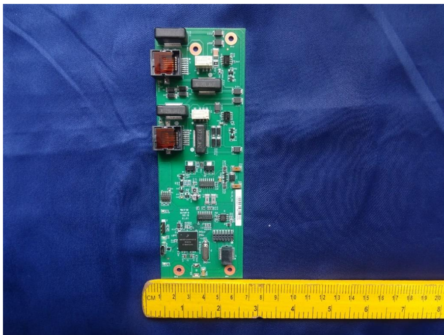
Photo 12: Pot PCB diemansional View
