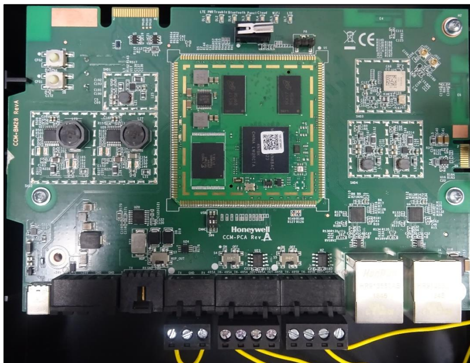
PCB FRONT VIEW
