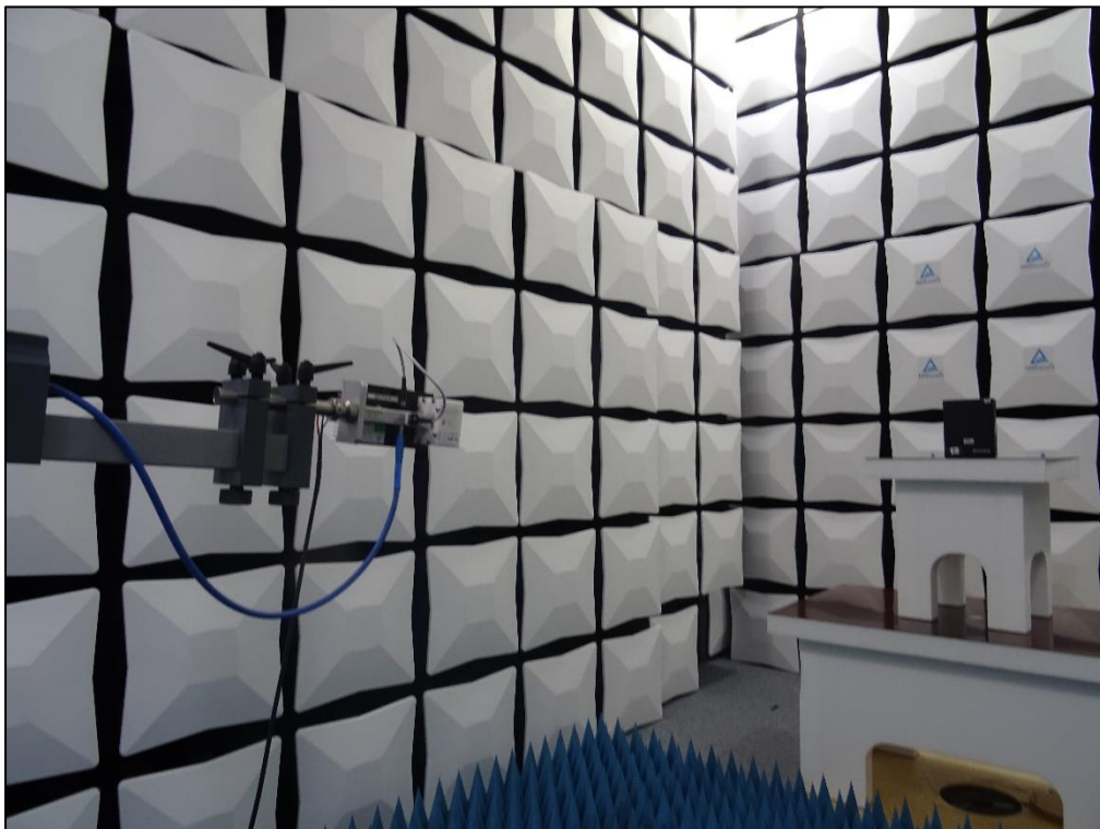
Frequency range:18-40GHz
