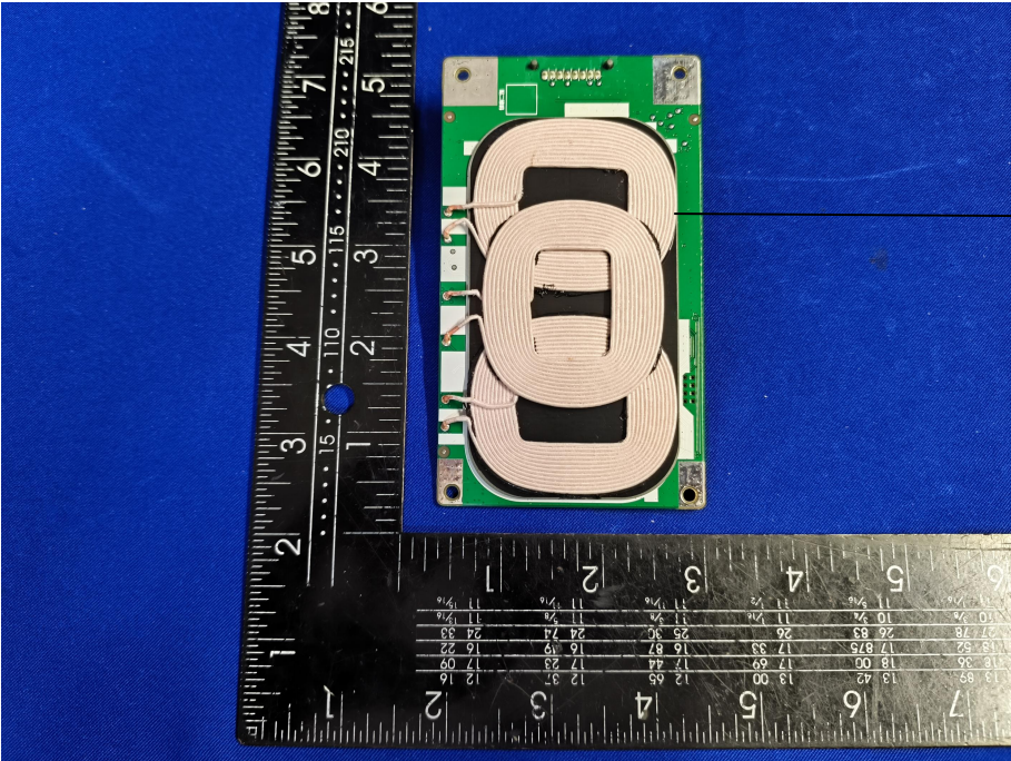
WPT Antenna
