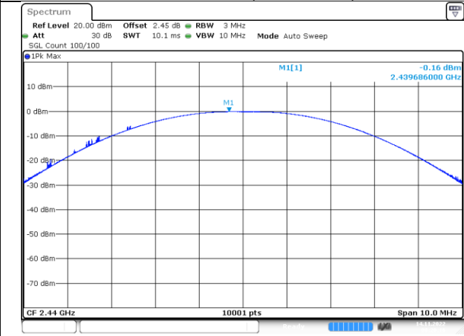
Channel 19 (2440MHz)
