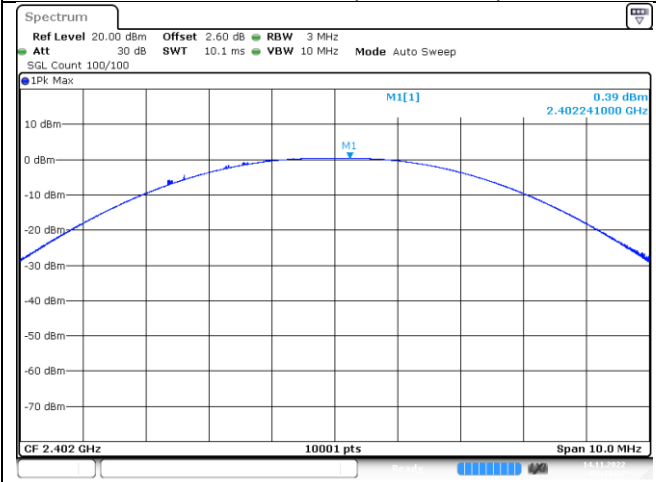
Channel 0 (2402MHz)
