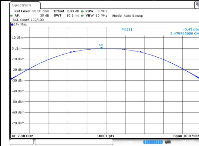
Channel 39 (2480MHz)
