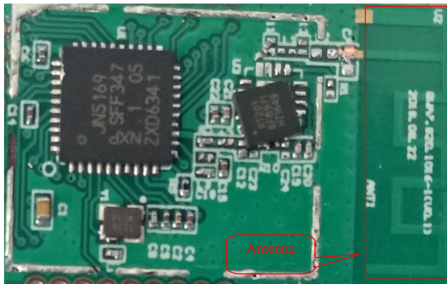
EUT – PCB Top Module View
