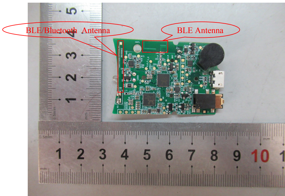
EUT – PCB Bottom View
