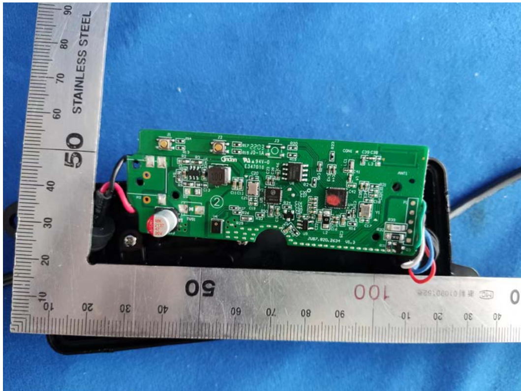
FIGURE 8 CYNC DIRECT CONNECTED OUTDOOR PREMIUM LIGHT STRIP (16FT.) (M/N: CLEDSTR36SCDODP) CHIP&CRYSTAL ON RBOARD
