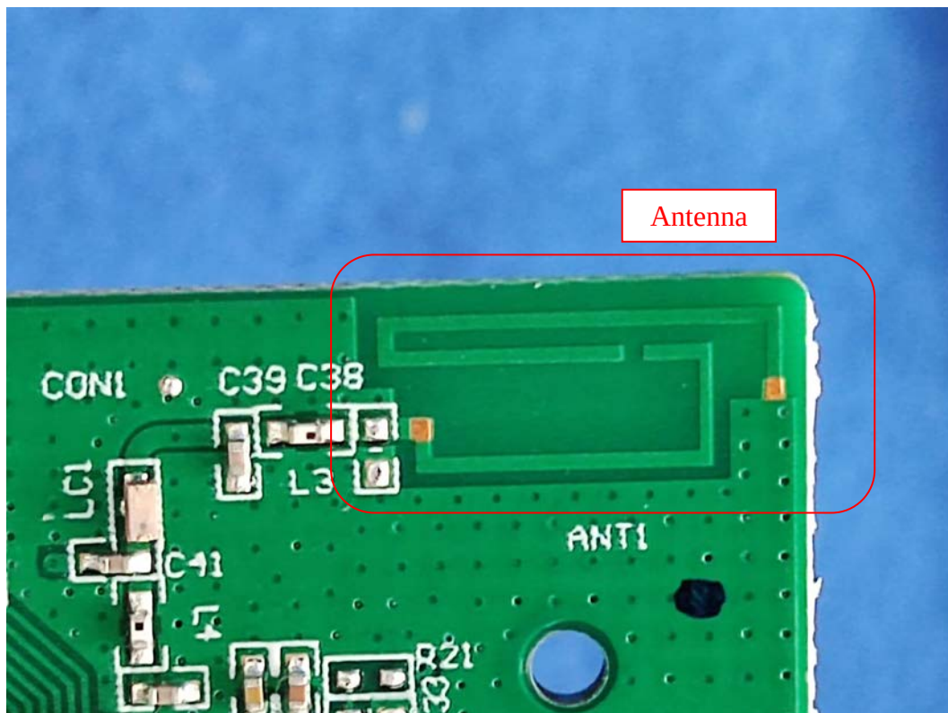
FIGURE 10 CYNC DIRECT CONNECTED OUTDOOR PREMIUM LIGHT STRIP (16FT.) (M/N: CLEDSTR36SCDODP) ANTENNA
