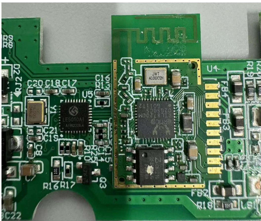
PCB view ( wireless module )
