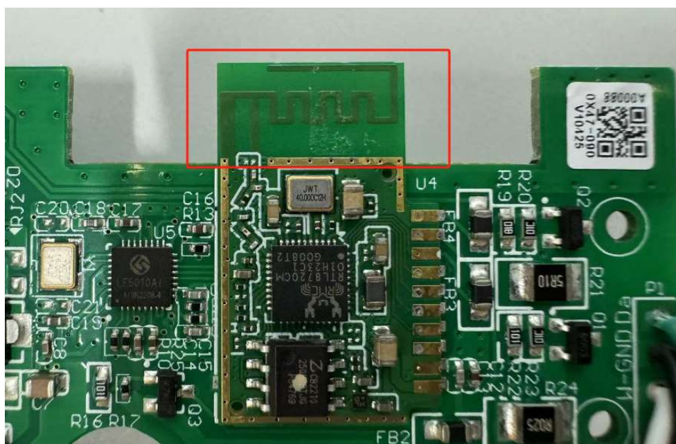
Wireless module Antenna
