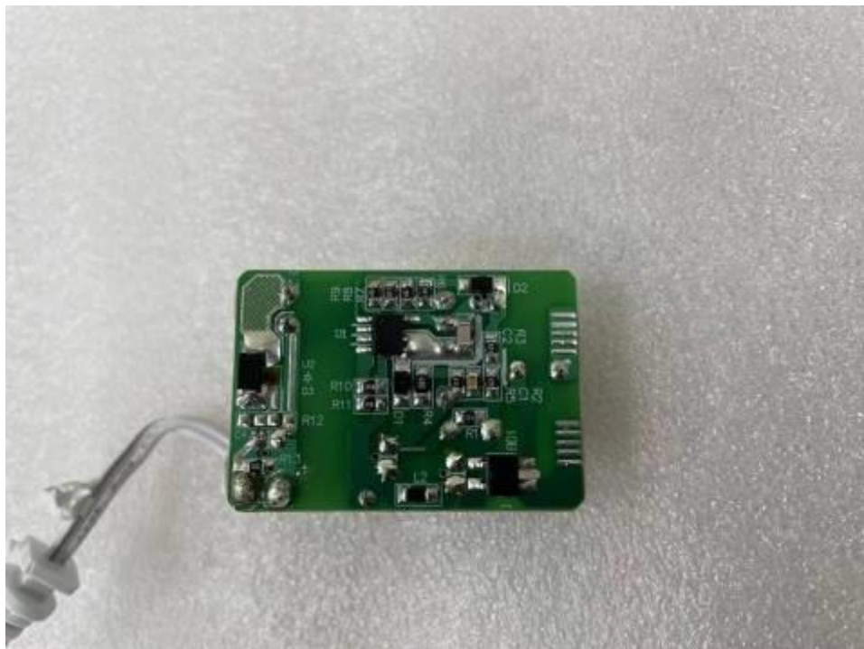
Driver PCB
