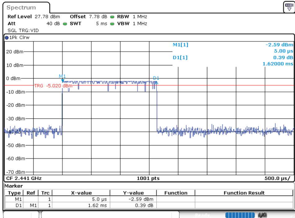
Dwell NVNT 1-DH5 2441MHz
