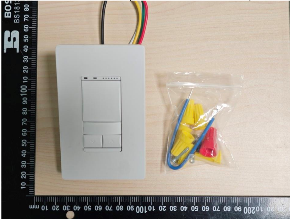
Motion Button Dimmer (HVIN: CSWDMOCK3T1/MSWF)
