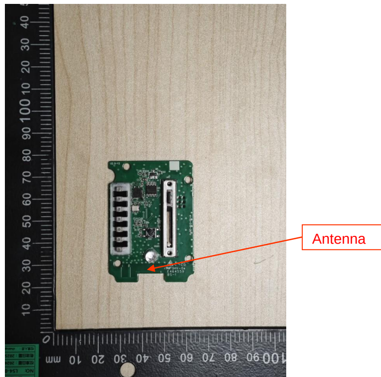
Internal View of EUT-4
