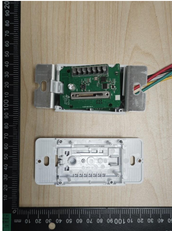
Internal View of EUT-1
