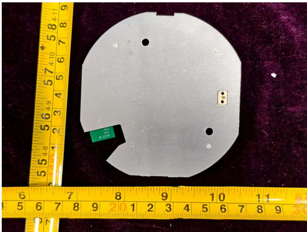
FIGURE 9 DOWNLIGHT (CFIXRSCR6CRVDMS) BOARD(BACK)
