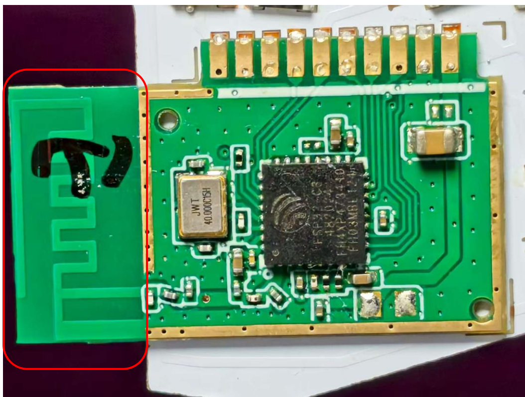
FIGURE 10 DOWNLIGHT (CFIXRSCR6CRVDMS) CHIP&CRYSTAL&ANTENNA
