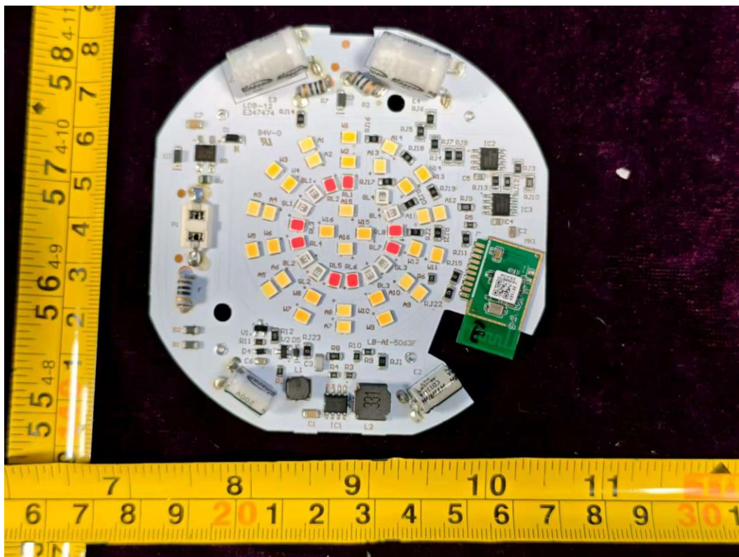
FIGURE 8 DOWNLIGHT (CFIXRSCR6CRVDMS) BOARD(FRONT)
