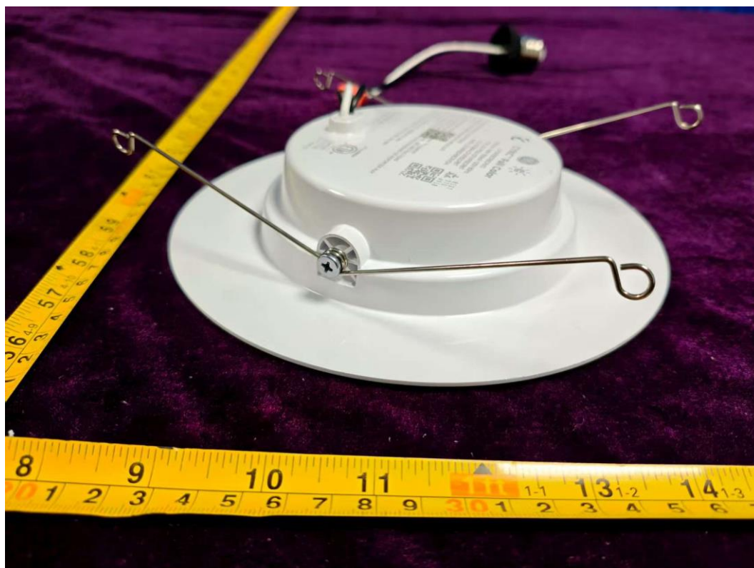
FIGURE 4 DOWNLIGHT (CFIXRSCR6CRVDMS) GENERAL VIEW(SIDE-2)
