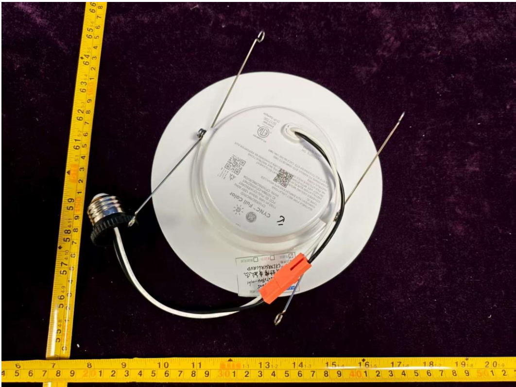
FIGURE 2 DOWNLIGHT (CFIXRSCR6CRVDMS) GENERAL VIEW(BOTTOM)
