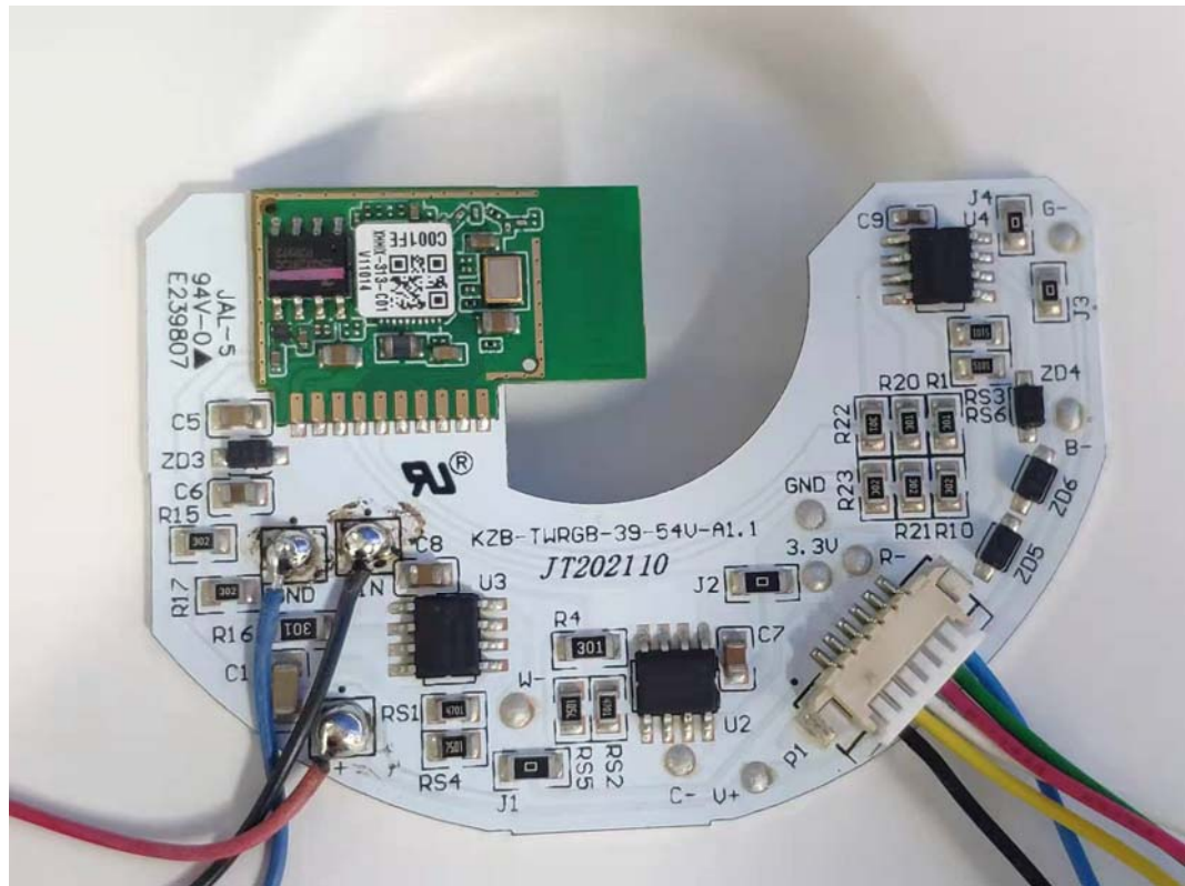
FIGURE 6 CYNC FIXTURE CANLESS (M/N: CFIXCNLR6C1) MAIN BOARD (SOLDERED SIDE)
