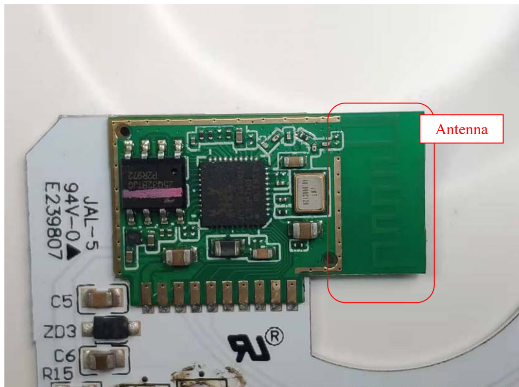
FIGURE 8 CYNC FIXTURE CANLESS (M/N: CFIXCNLR6C1) POWER BOARD (COMPONENT SIDE)
