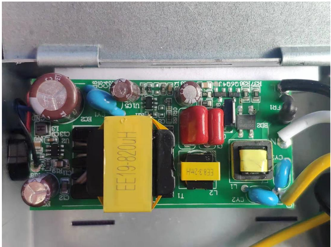
FIGURE 10 CYNCR FIXTURE CANLESS (M/N: CFIXCNLR4S1) COVER REMOVED #2
