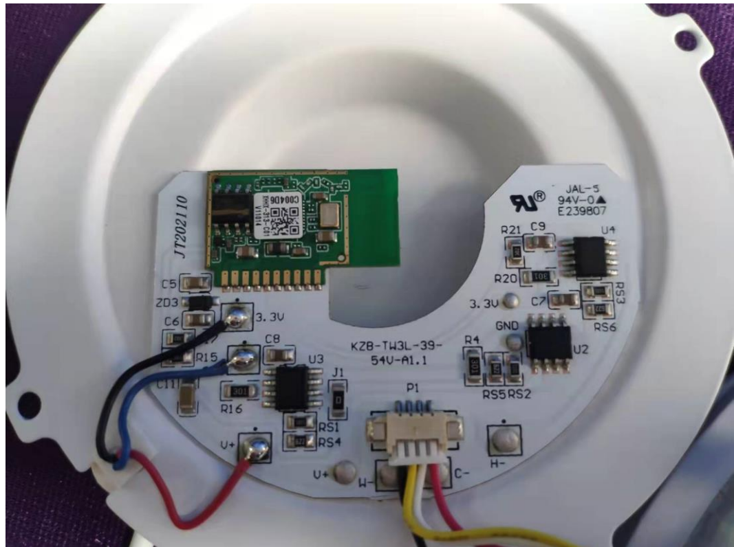
FIGURE 6 CYNC FIXTURE CANLESS (M/N: CFIXCNLR4S1) MAIN BOARD (SOLDERED SIDE)
