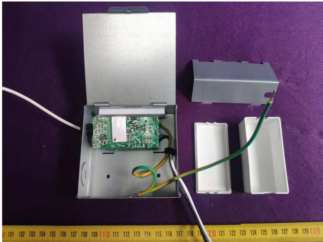
FIGURE 4 CYNCR FIXTURE CANLESS (M/N: CFIXCNLR4S1) COVER REMOVED #1
