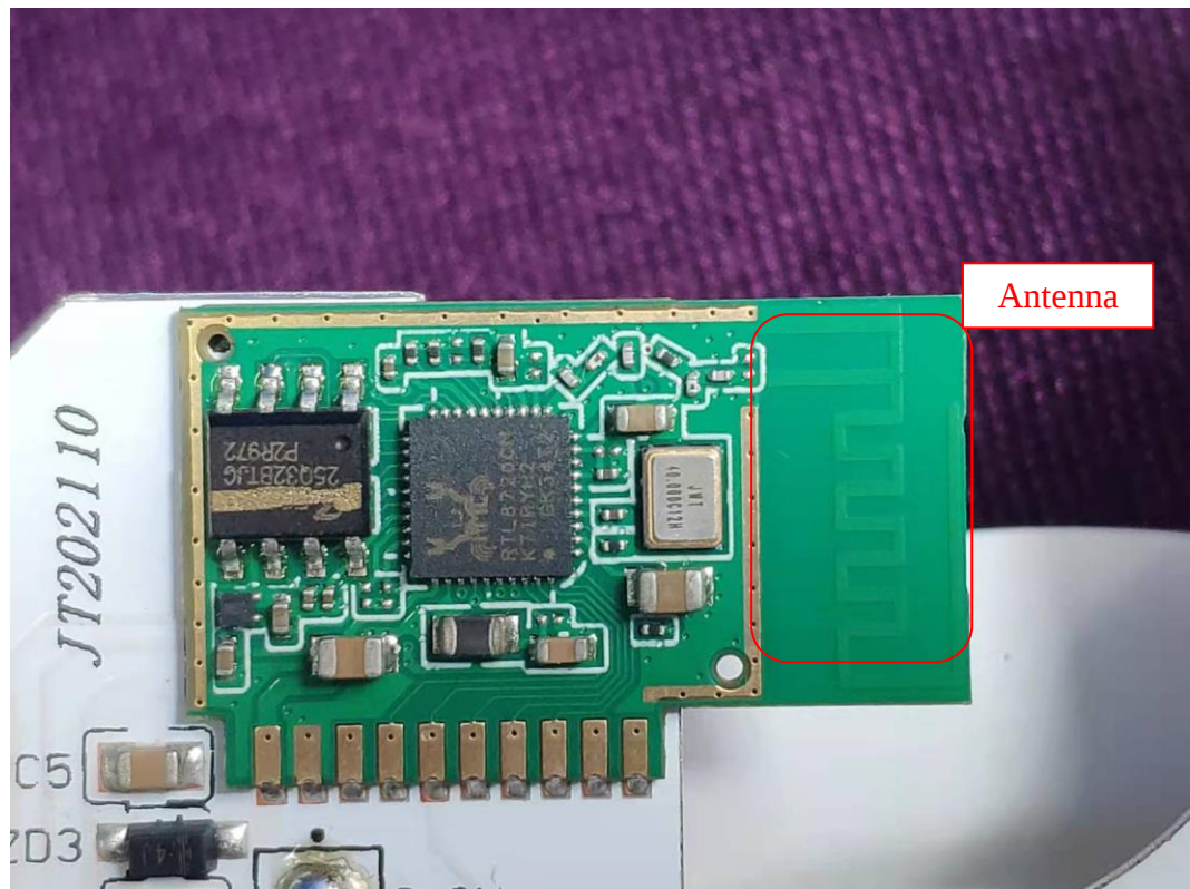
FIGURE 8 CYNC FIXTURE CANLESS (M/N: CFIXCNLR4S1) POWER BOARD (COMPONENT SIDE)
