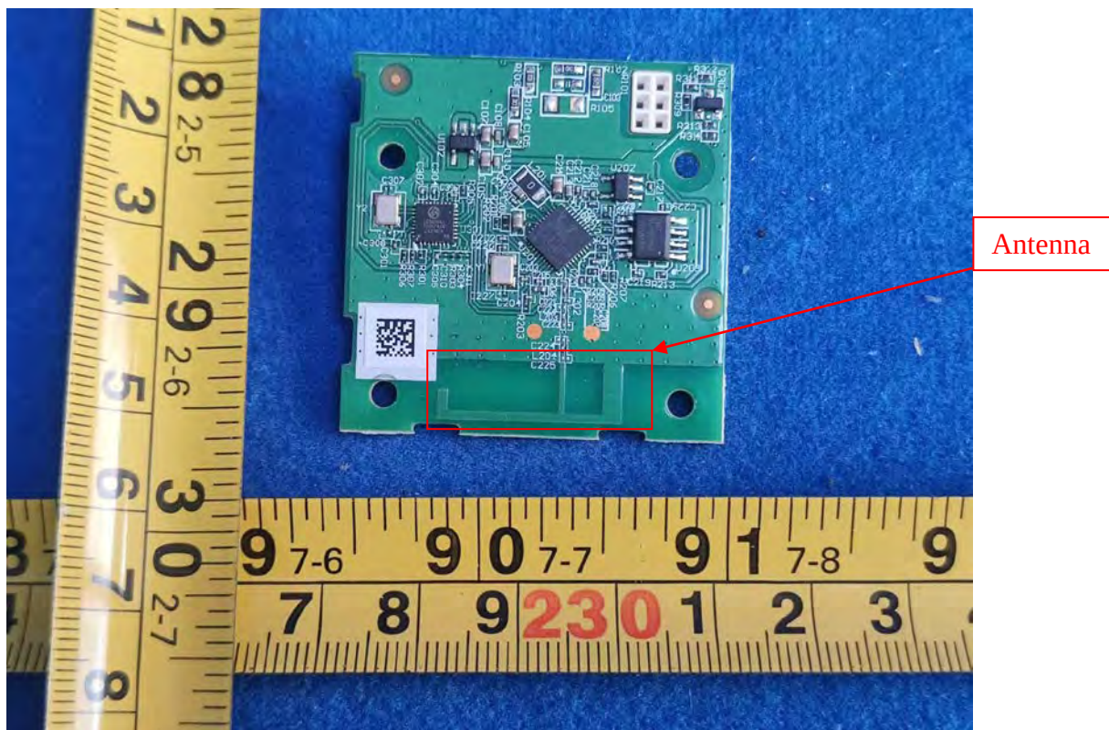
FIGURE 14 CYNIC DYNAMIC EFFECTS SMART CAFÉ LIGHTS (M/N: CCF48CDOD/ENS) RF BOARD BACK
