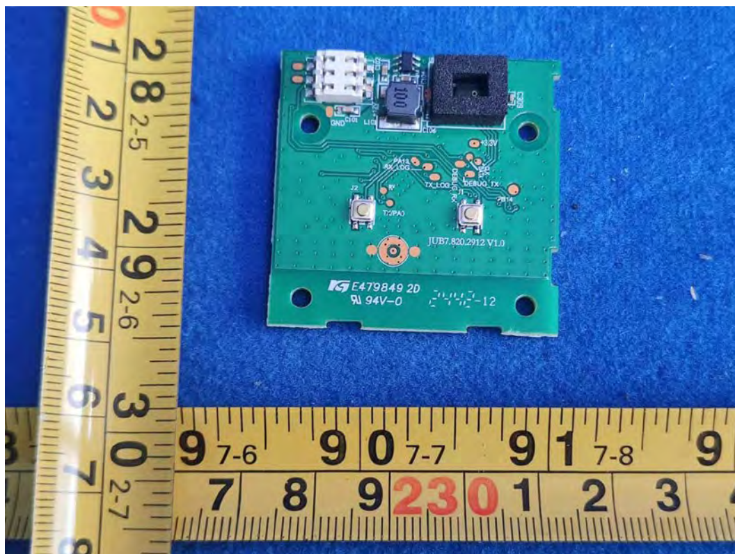
FIGURE 14 CYNIC DYNAMIC EFFECTS SMART CAFÉ LIGHTS (M/N: CCF48CDOD/ENS) RF BOARD BACK
