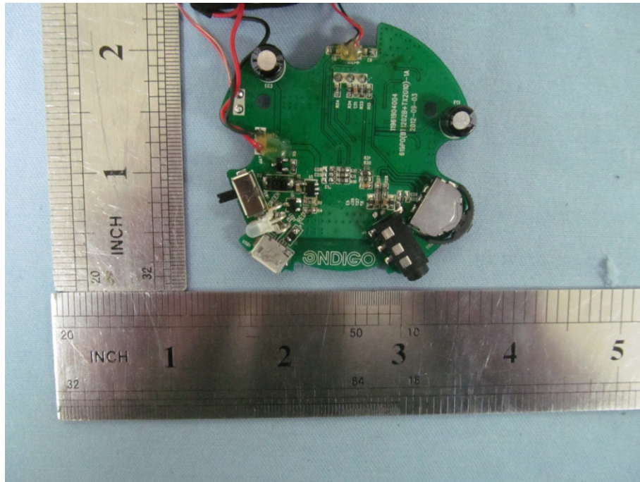
BACK VIEW OF PCB-1
