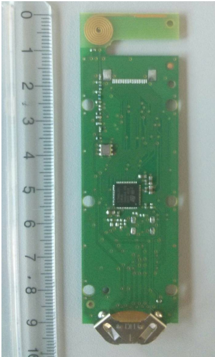
Figure 7.4 Component Side (5 Channel, 2008806)
