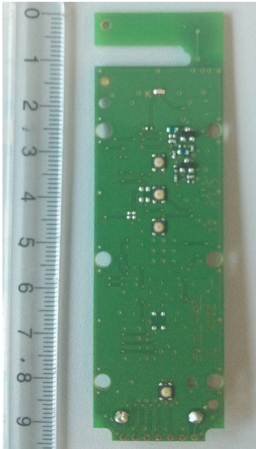
Figure 7.5 Foil Side (5 Channel, 2008806)
