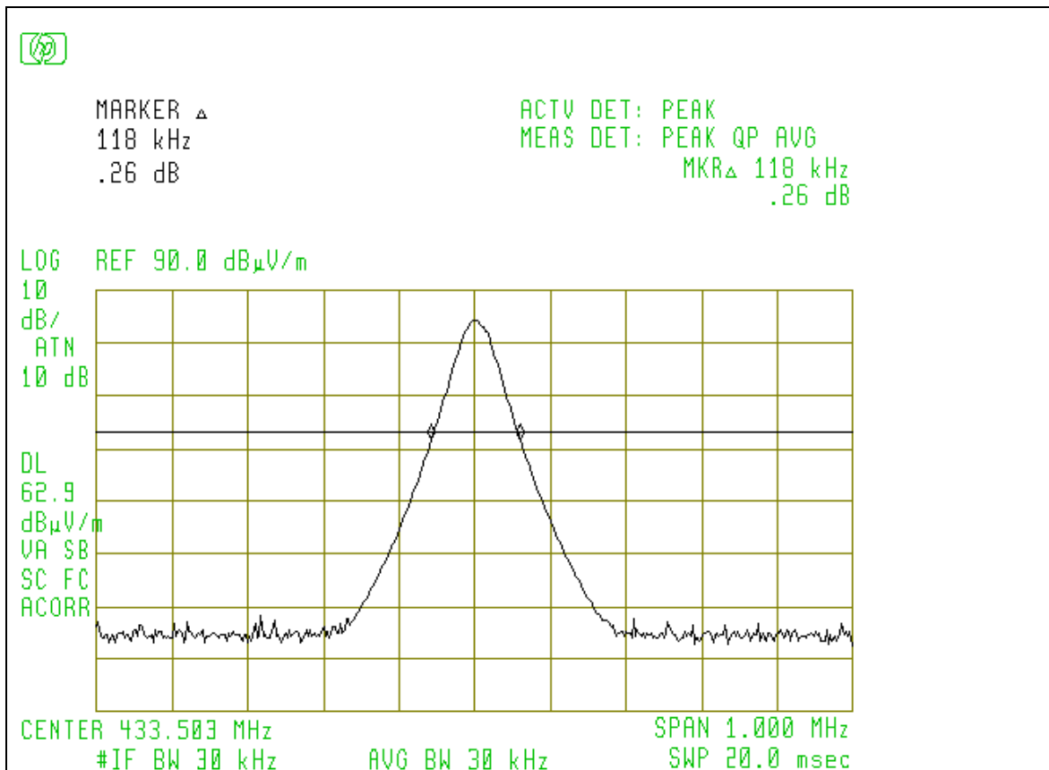
Figure 6.1 20 dB Occupied Bandwidth
