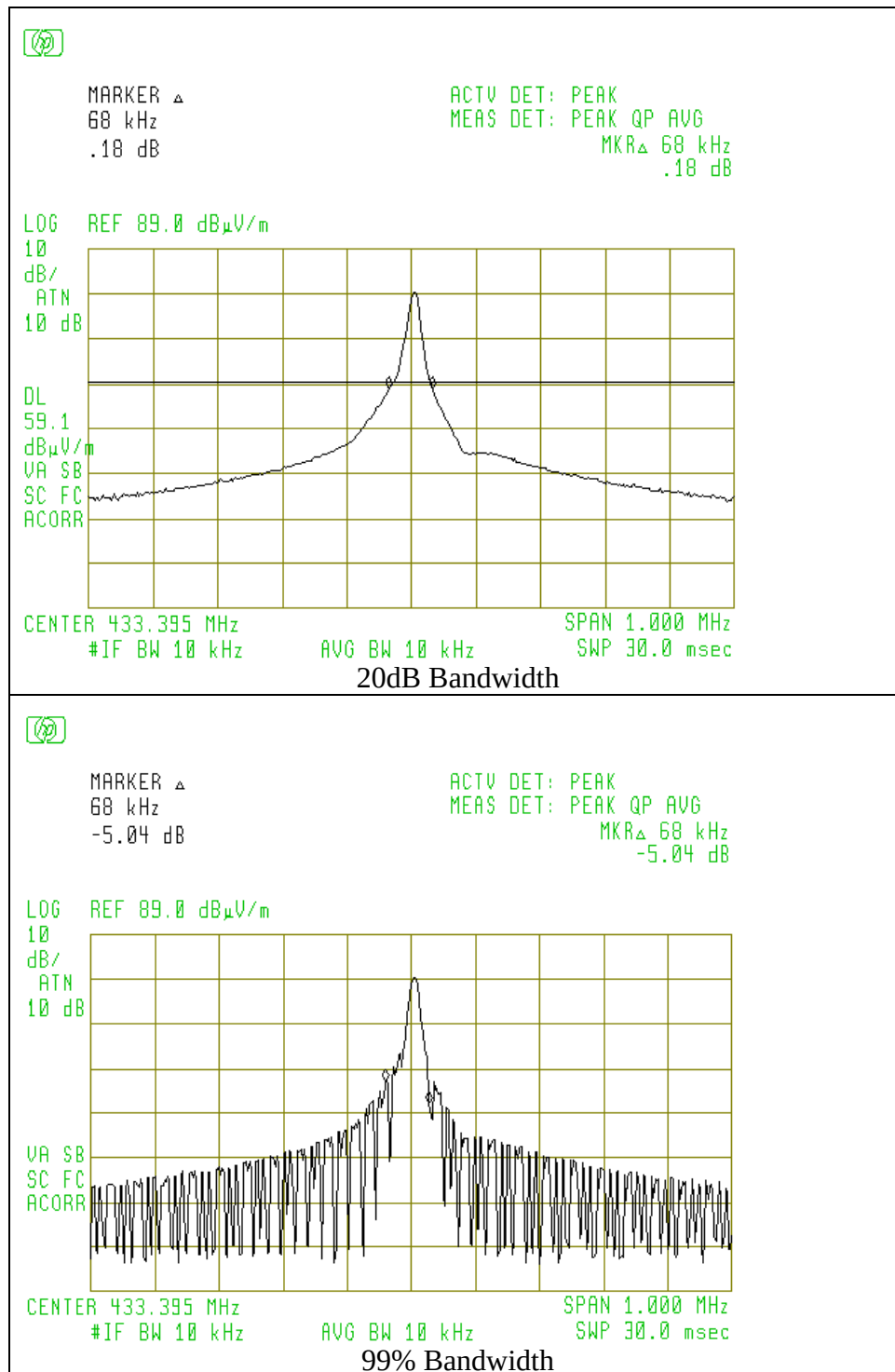
Figure 6.1 Occupied Bandwidth
