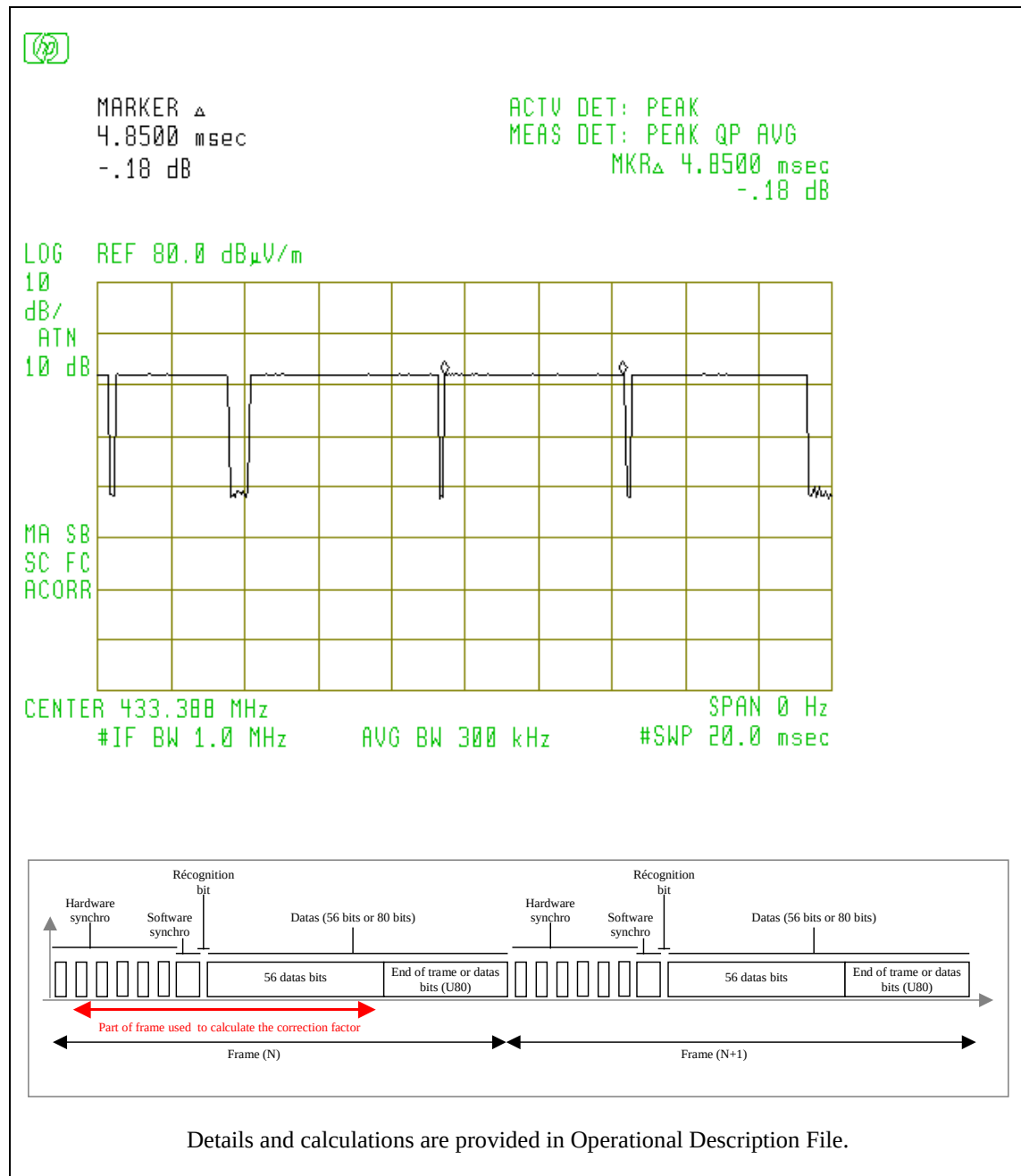
Figure 6.2 Pulse Train Timing
