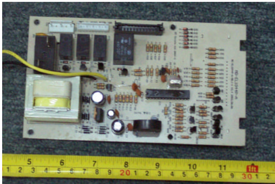
PCB 1 Front
