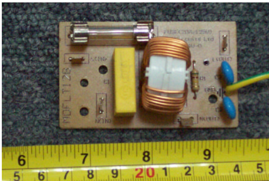
PCB 2 Front
