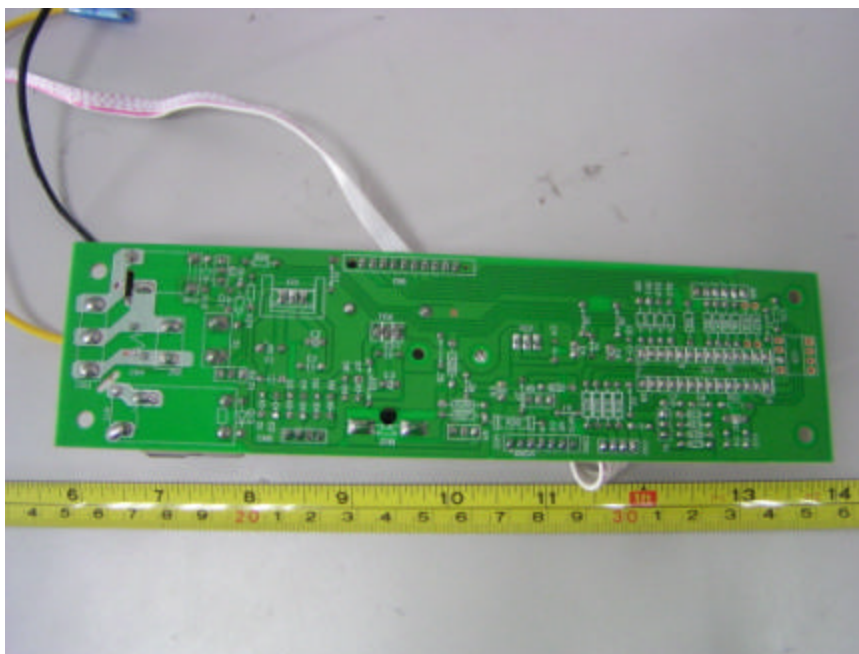
EUT – Solder View (4)
