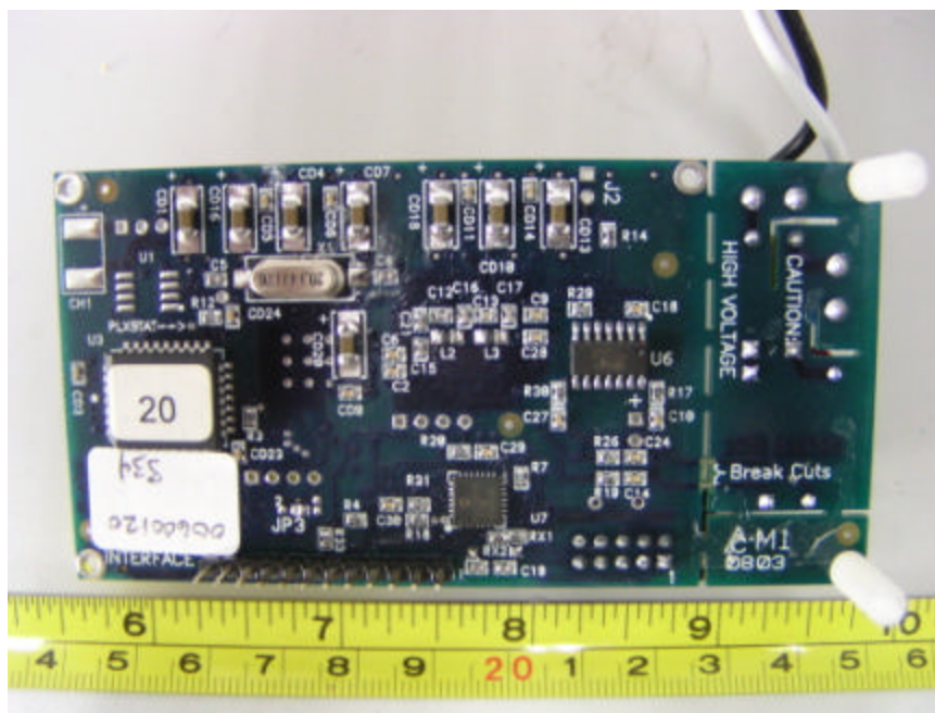
EUT – Solder View (3)
